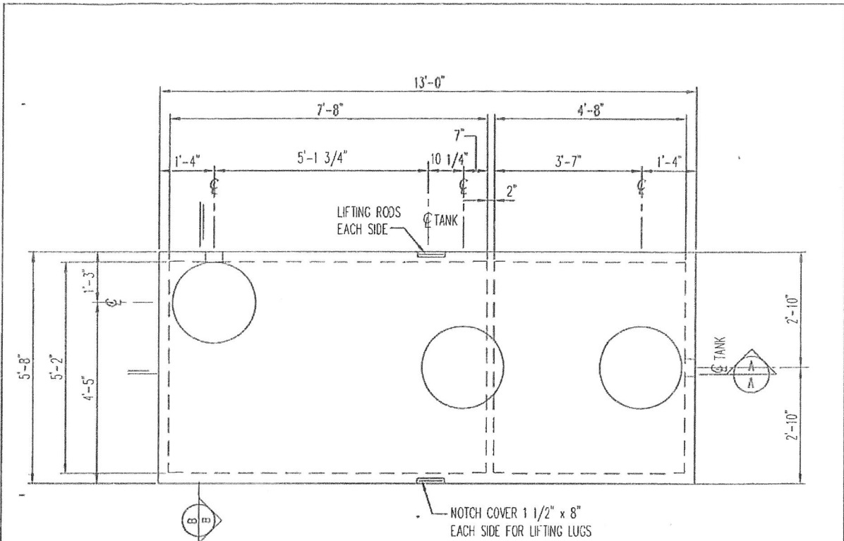
1600 GALLON 2 COMP. TANK 1/2" = 1'-0"
