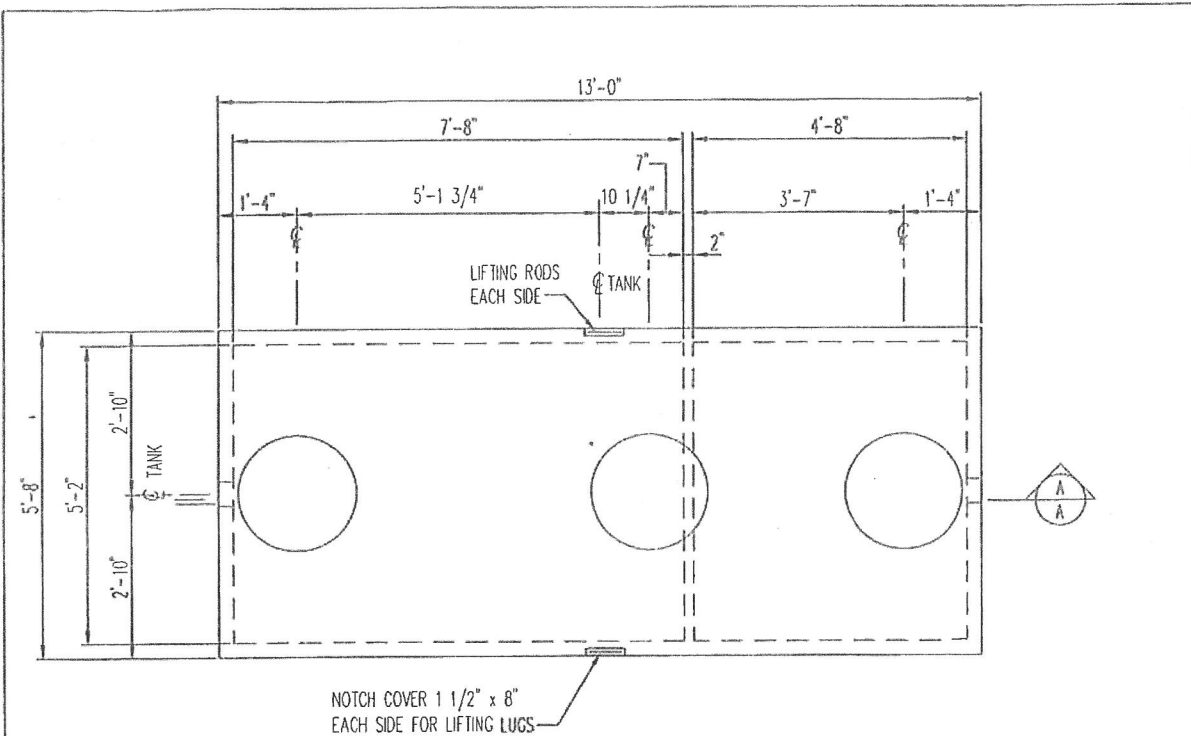
1600 GALLON 2 COMP. TANK 1/2" = 1'-0"
