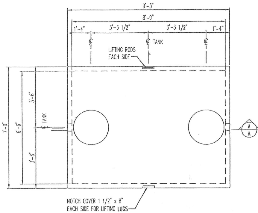
1000 GALLON LOW PROFILE TANK 1/2" = 1'-0"
