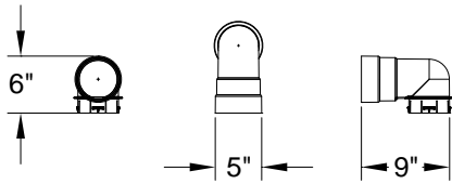
Quick4 Plus All-in-One Periscope
