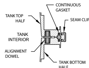
MID-HEIGHT SEAM SECTION DETAIL
