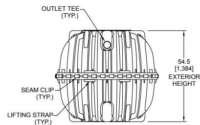
END VIEW
