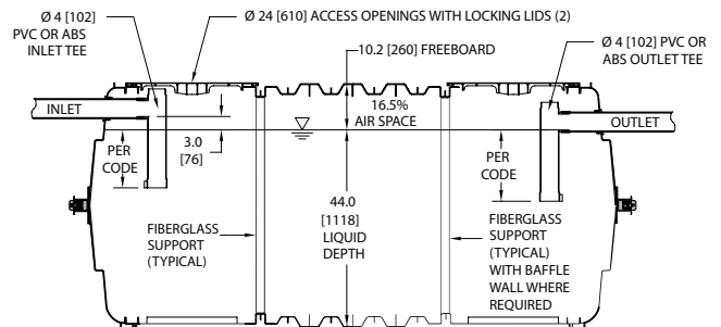
SIDE VIEW
