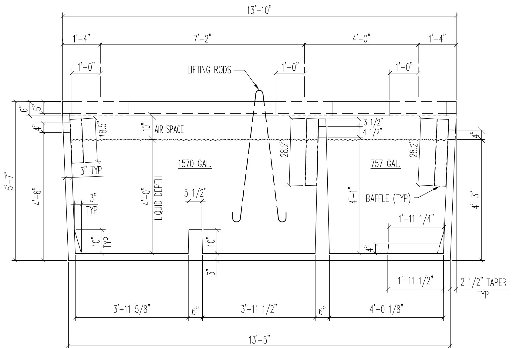
SECTION 1/2" = 1'-0"
