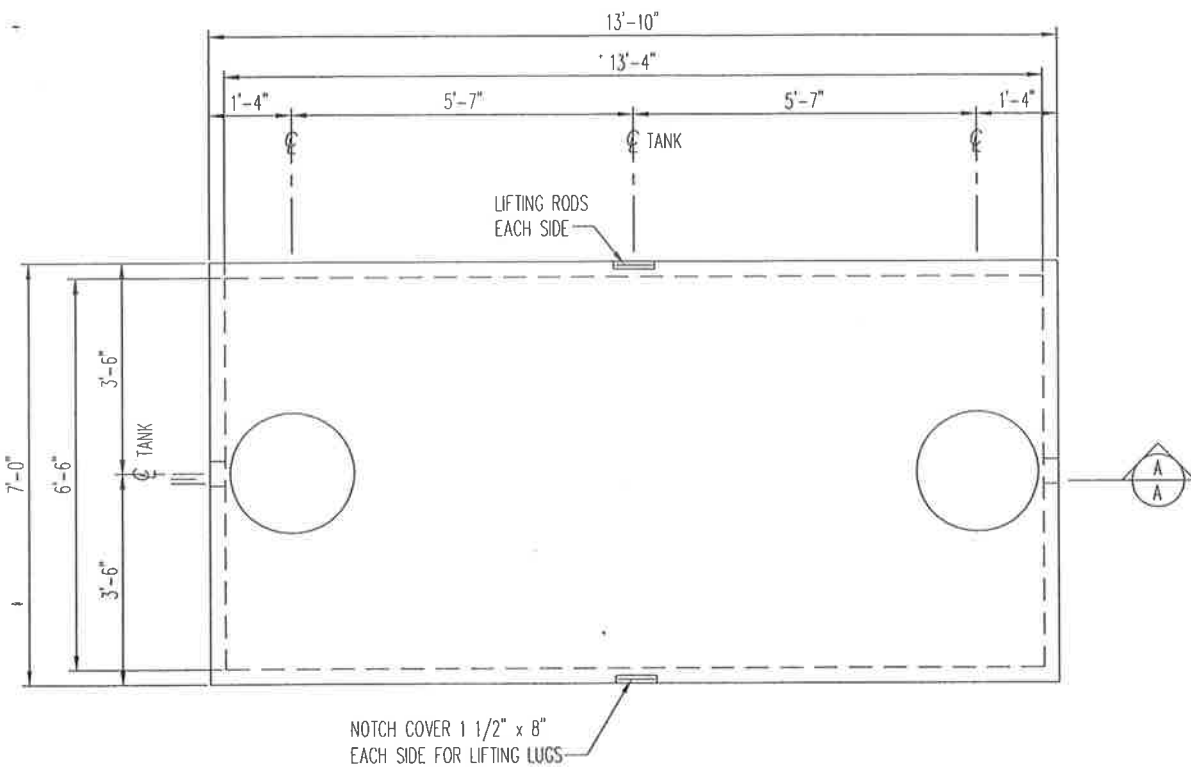
2000 GALLON TANK 1/2" = 1'-0"
