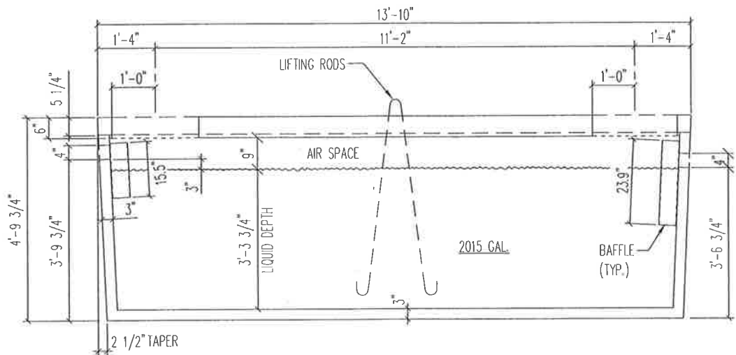
SECTION A-A 1/2" = 1'-0"
