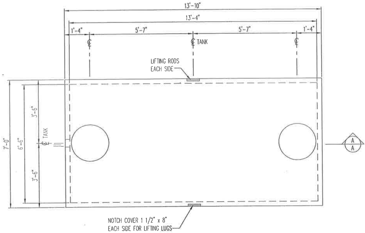
2000 GALLON TANK 1/2" = 1'-0"
