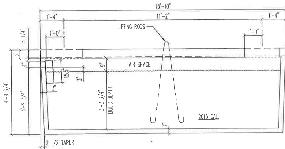
SECTION 1/2" = 1'-0"
