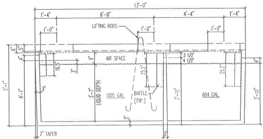
SECTION 1/2" = 1'-0"
