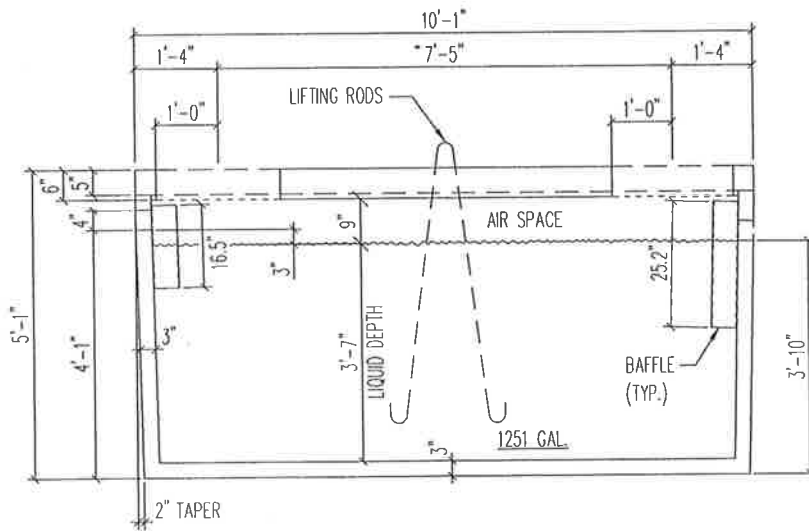
1250 GALLON TANK 1/2" = 1'-0"
