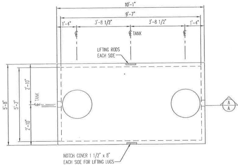
1250 GALLON TANK 1/2" = 1'-0"
