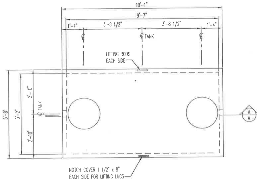
1250 GALLON TANK 1/2" = 1'-0"
