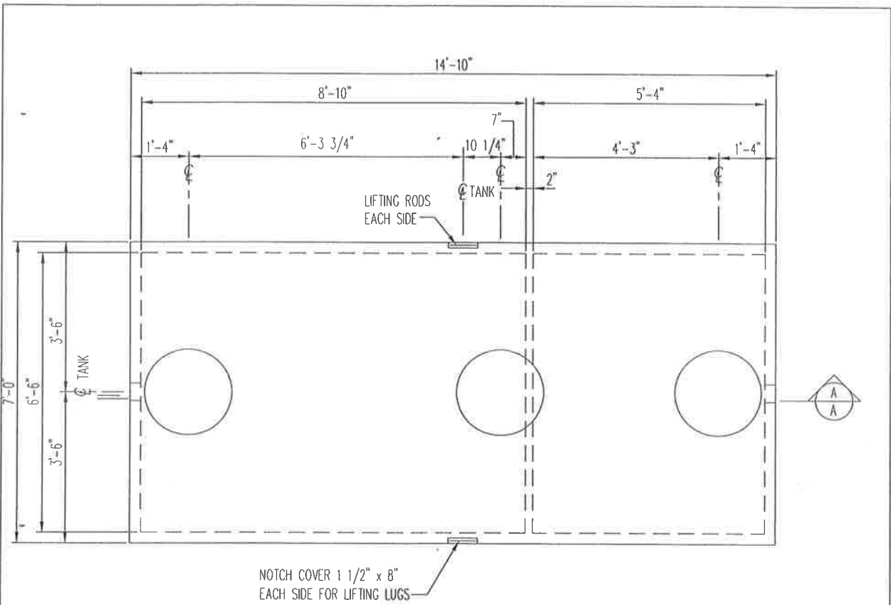
1600 GALLON 2 COMP. LOW PROFILE TANK 1/2" = 1'-0"
