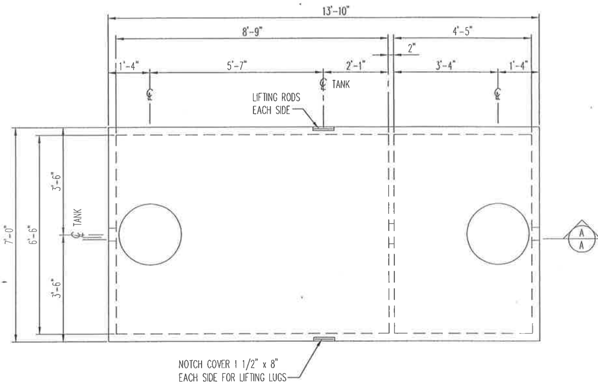
1500 GALLON LOW PROFILE TANK w/MOLE HOLE 1/2" = 1'-0"
