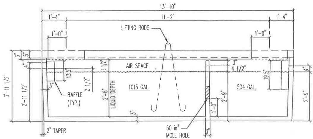
SECTION A-A 1/2" = 1'-0"
